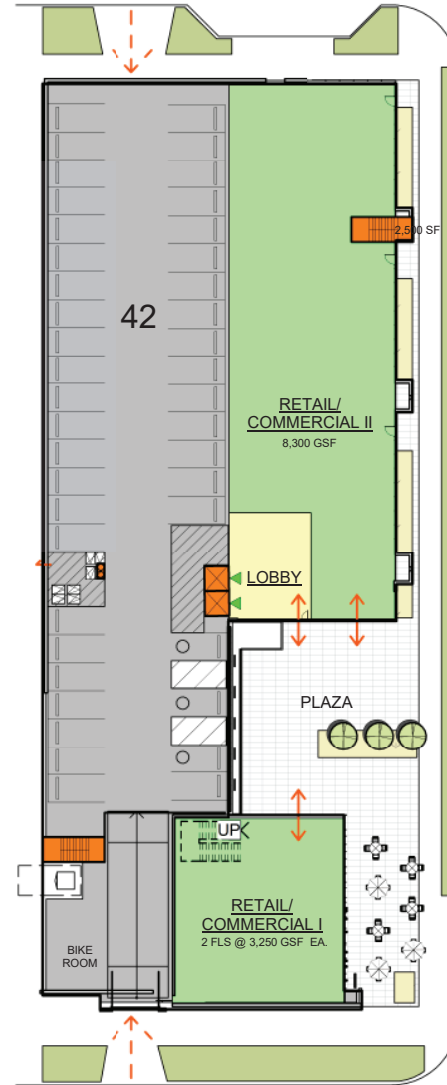
O2.2 - LEVEL 1 PLAN 29,600 GSF
